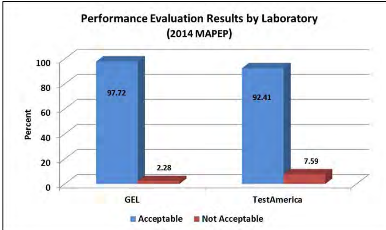
FIGURE 13.2 — 2014 MAPEP Results
