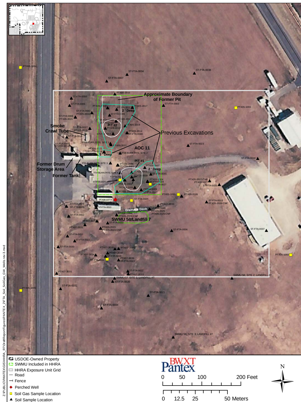
Figure F-1. FTA Sample Locations and Exposure Area Grid Configuration
