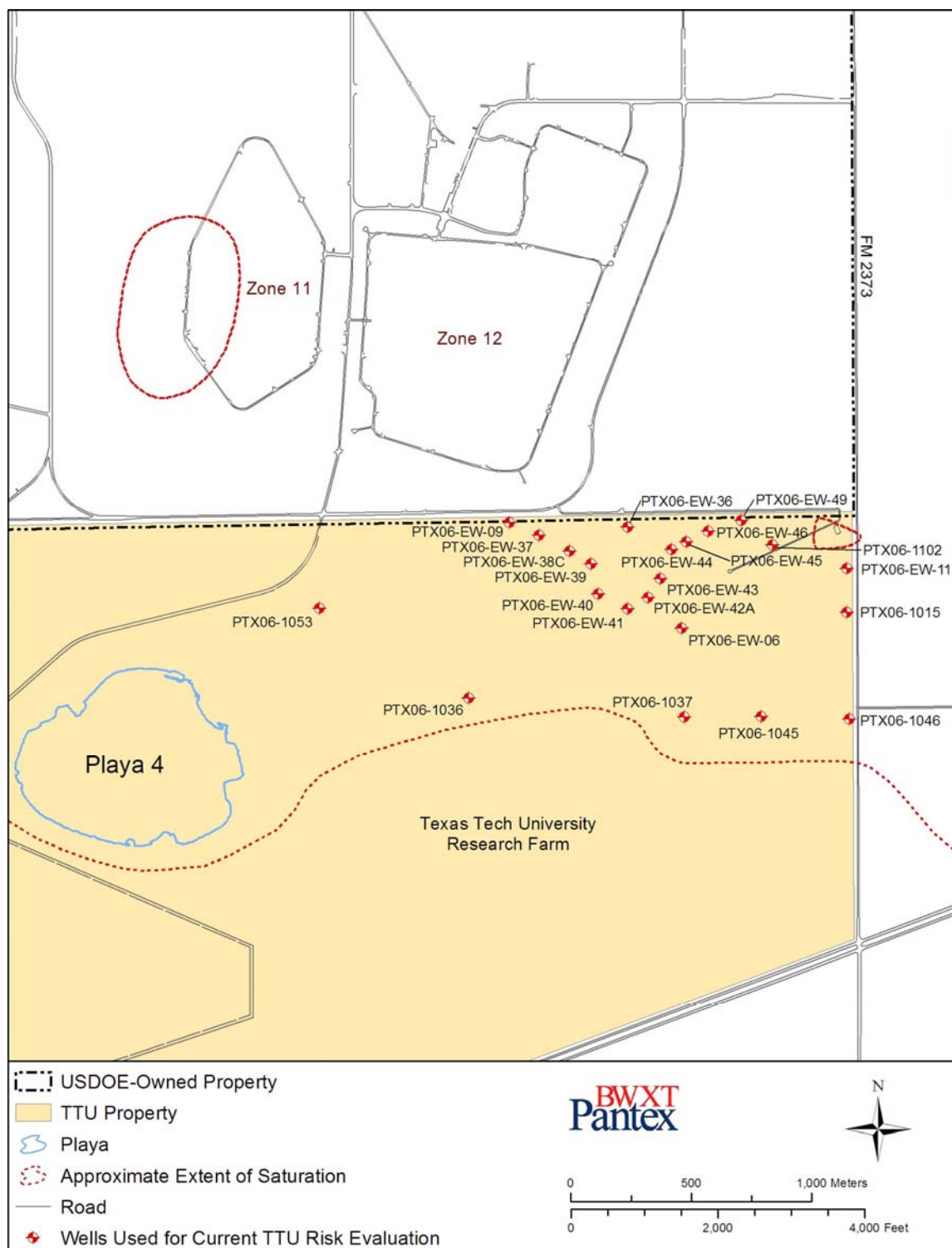
Figure H-2. Wells Used for Evaluation of Current TTURF Perched Groundwater
