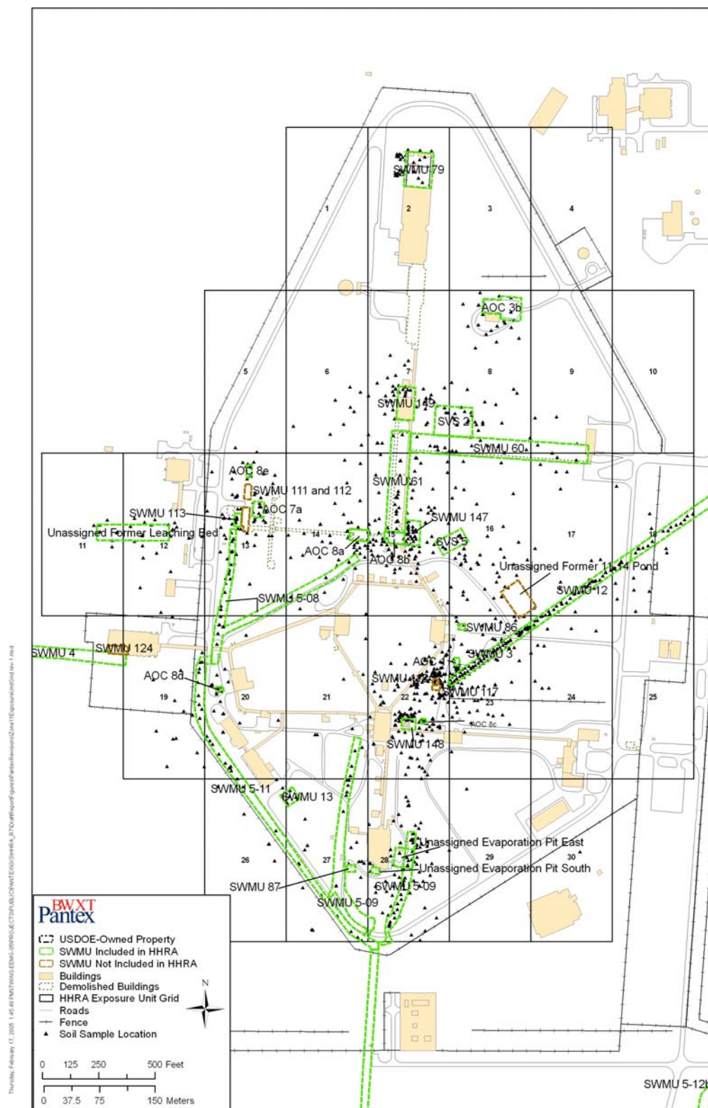
Figure D-1. Zone 11 Release Units and Exposure Area Grids
