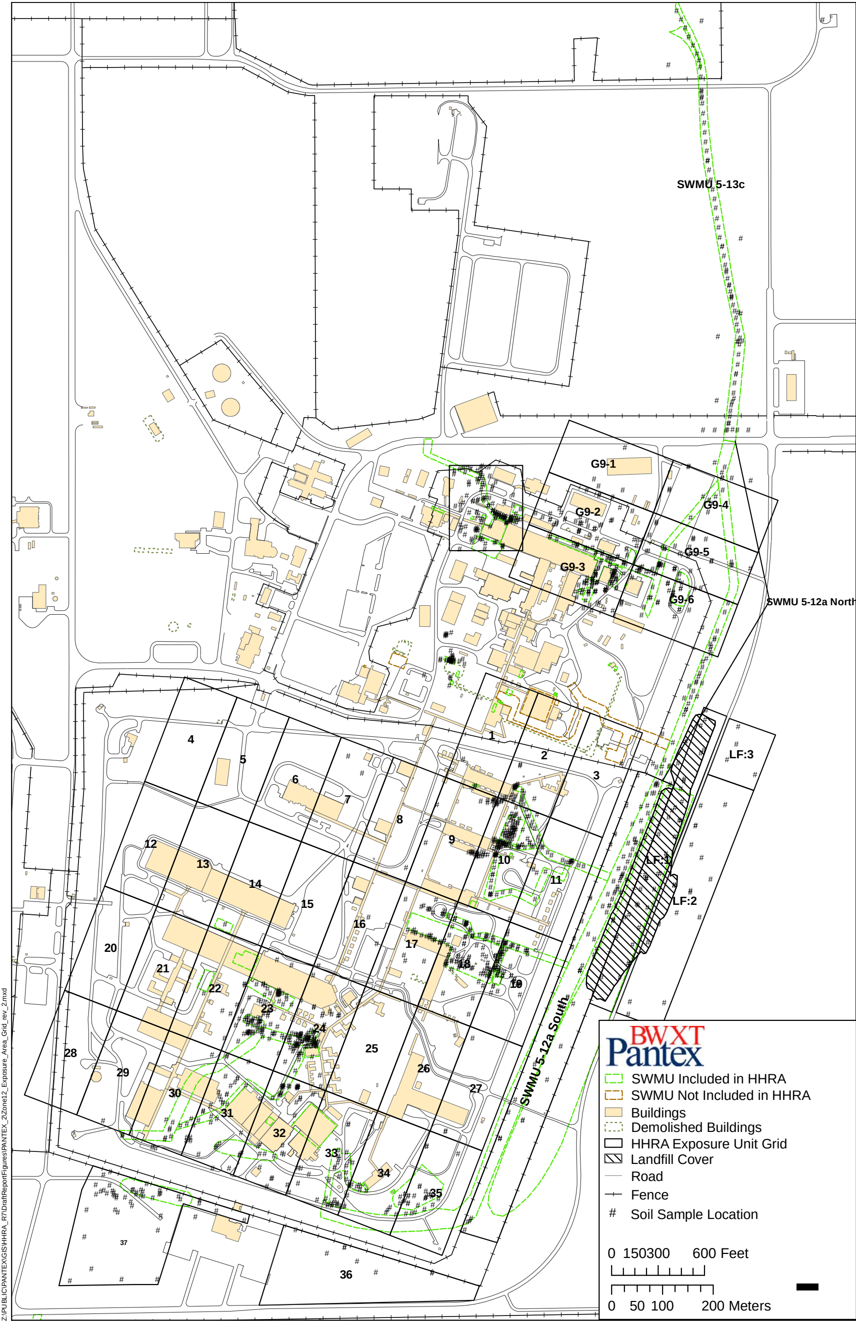
Figure E-2. Zone 12 Exposure Area Grid
