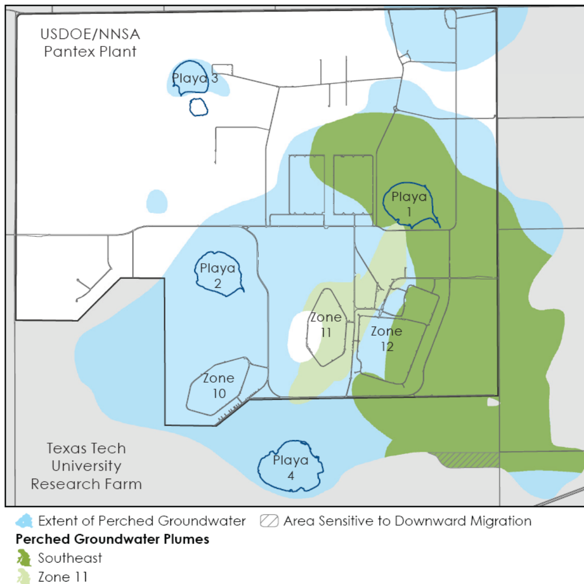
Figure H-1. Zone 11 and Zone 12 (Southeast) Perched Groundwater Plumes
