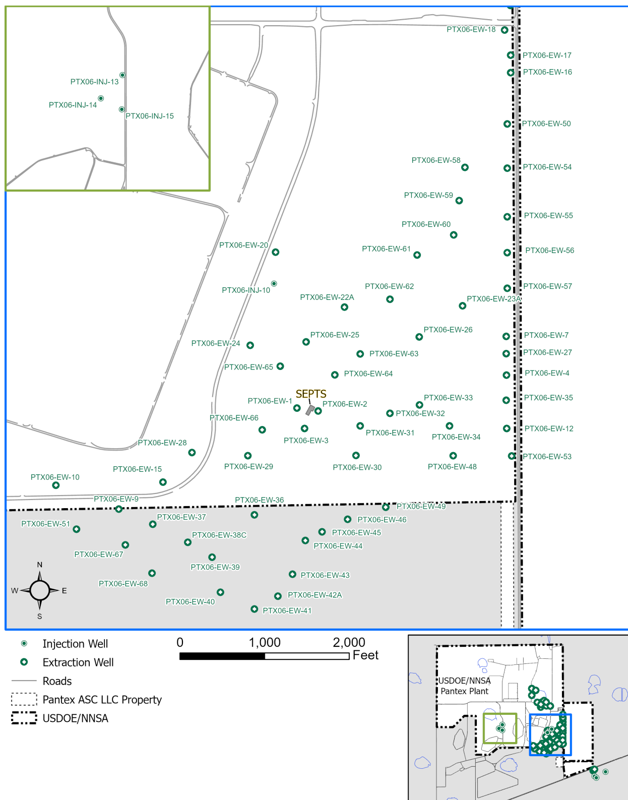
Fig. 1-16. SEPTS wells.
