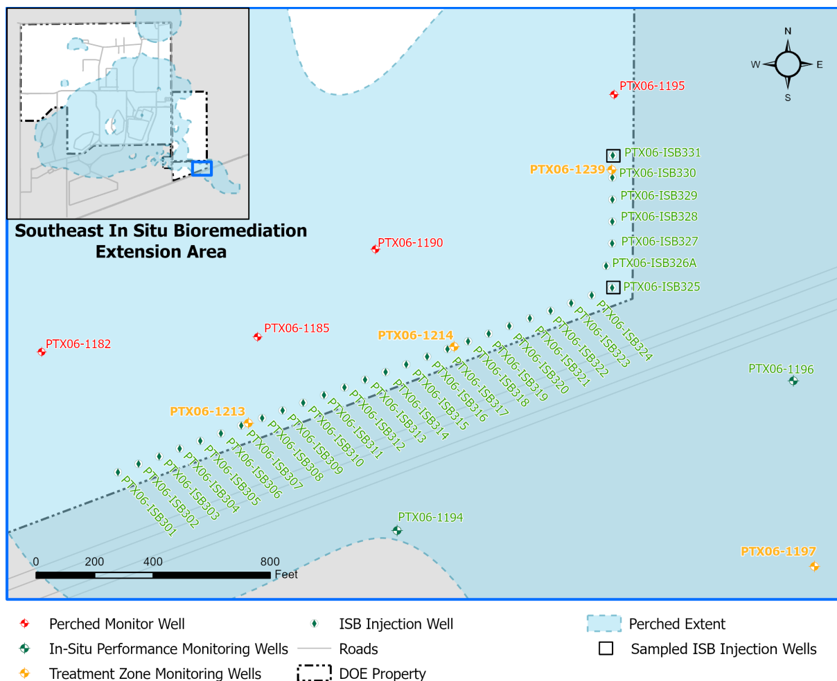
Fig. 1-11. Southeast ISB Extension treatment zone and performance monitoring wells.
