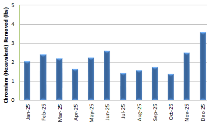
Fig. 2-13. SEPTS chromium mass removal by month.
