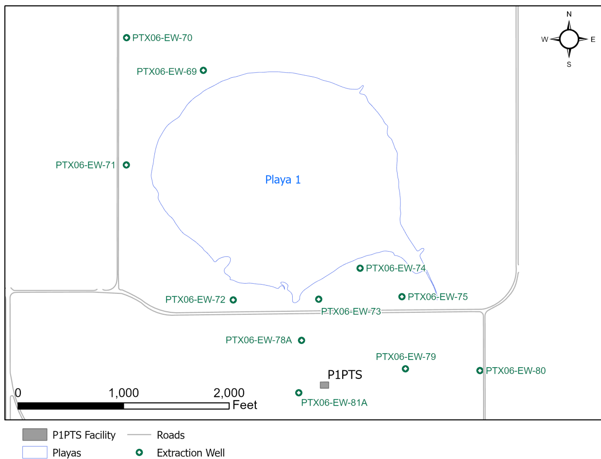
Fig. 1-17. P1PTS wells.
