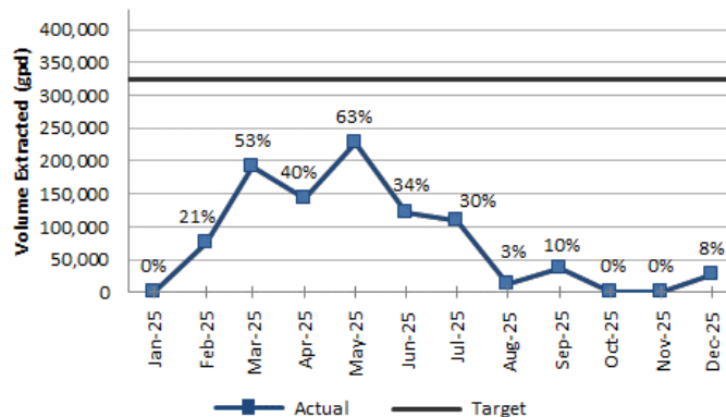
Fig. 2-4. P1PTS average GPD and % capacity.
