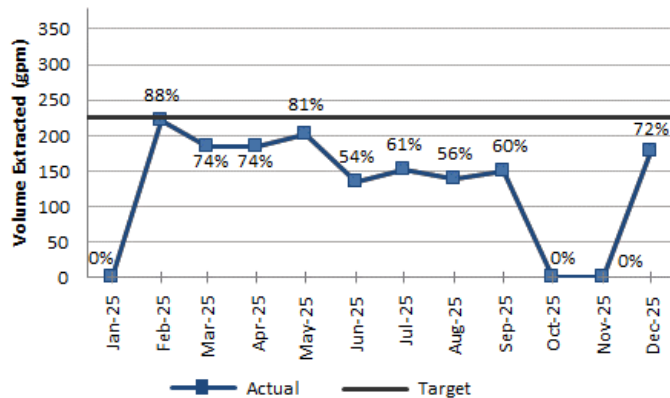
Fig. 2-2. P1PTS average GPM and % capacity.
