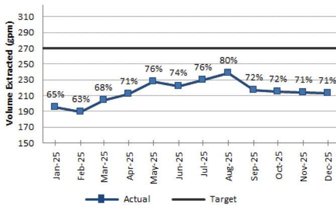
Fig. 2-8. SEPTS average GPM and % capacity.
