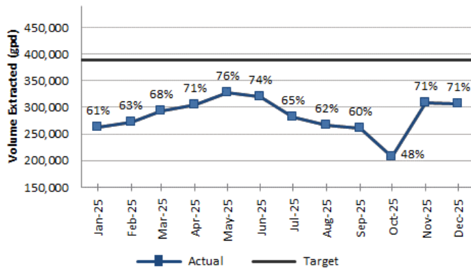
Fig. 2-11. SEPTS average GPD and % capacity.
