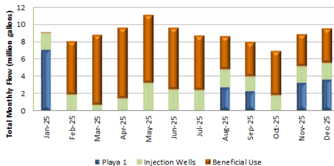
Fig. 2-12. SEPTS total flow volume and disposition of effluent.
