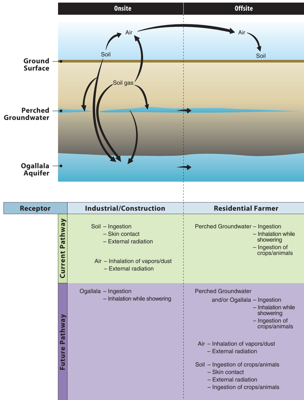
Generalized conceptual site model for Pantex Plant
